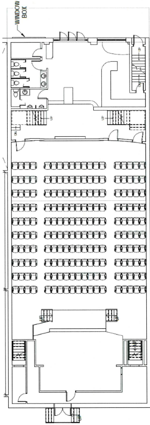
1 3/32" = 1'-0" N↑ EXISTING FIRST FLOOR
